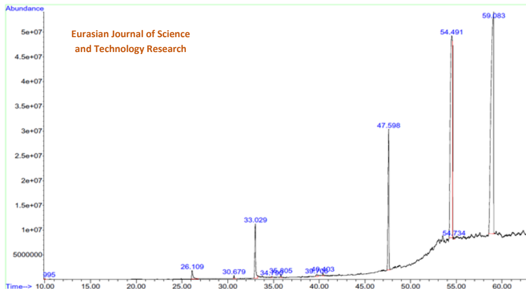
Figure 5 Gas chromatographic analysis of the extracted extract by USC-CO 2
