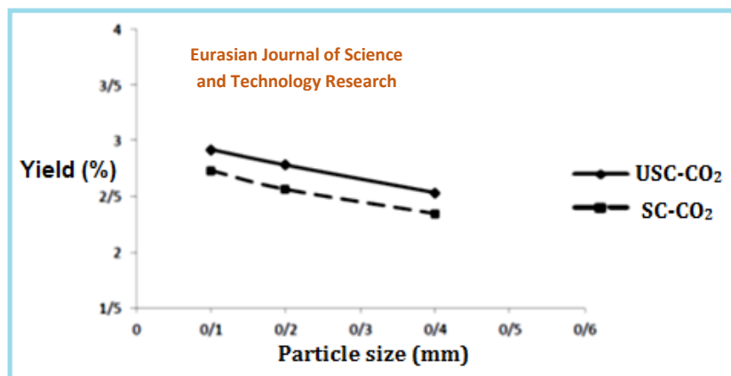
Figure 8 Effect of particle size on the yield of Oliveria decumbens extract at 180 bar and 65 °C
