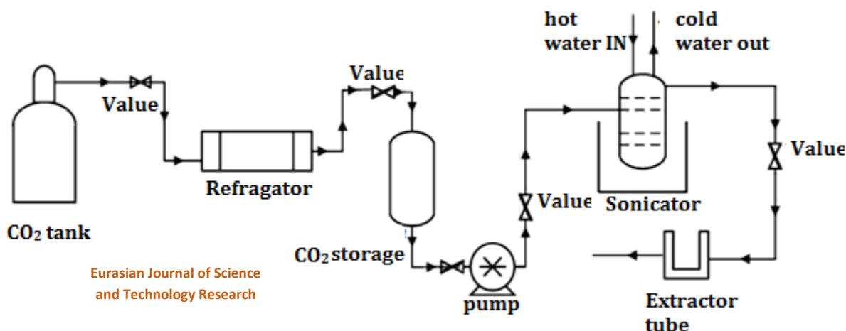
Figure 3 Diagram of a supercritical extraction device
