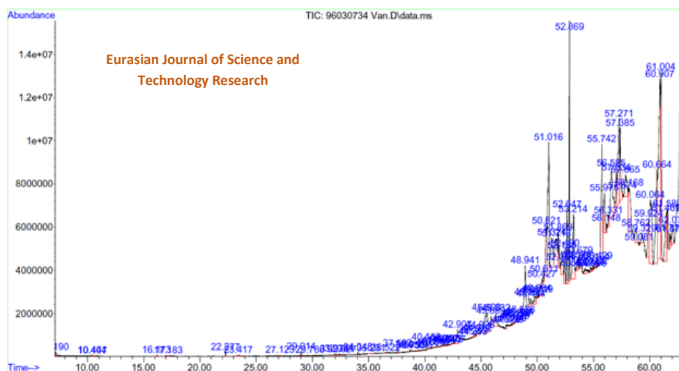
Figure 4 Gas chromatographic analysis of the extracted extract by SC-CO 2 method
