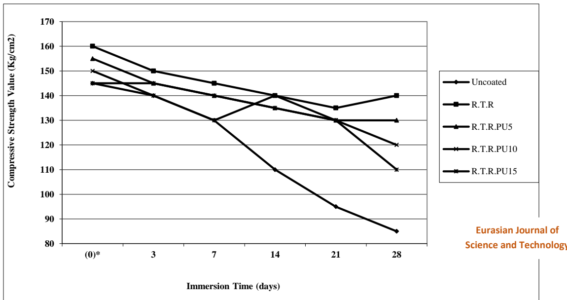
Figure 5 Effect of Tap Water on the Compressive Strength Values of Mortar Cubes Coated with Unmodified and Modified T.R
