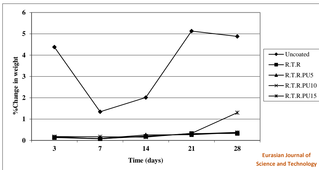
Figure 2 % Change in Weight for Mortar Cubes Coated with Unmodified and Modified T.R after Immersion in Tap Water
