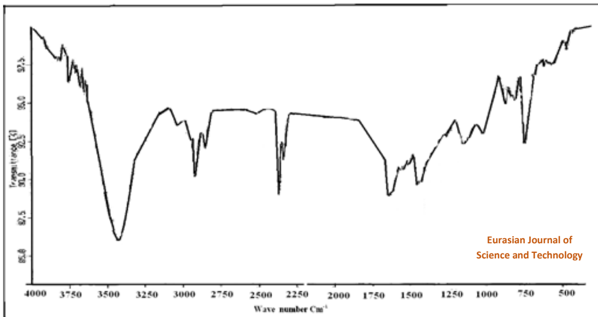
Figure 1 FTIR Spectrum of waste tar pitch
