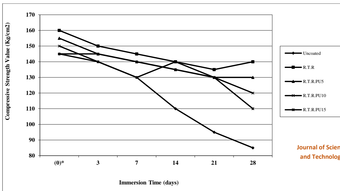
Figure 5. Effect of Tap Water on the Compressive Strength Values of Mortar Cubes Coated with Unmodified and Modified T.R
